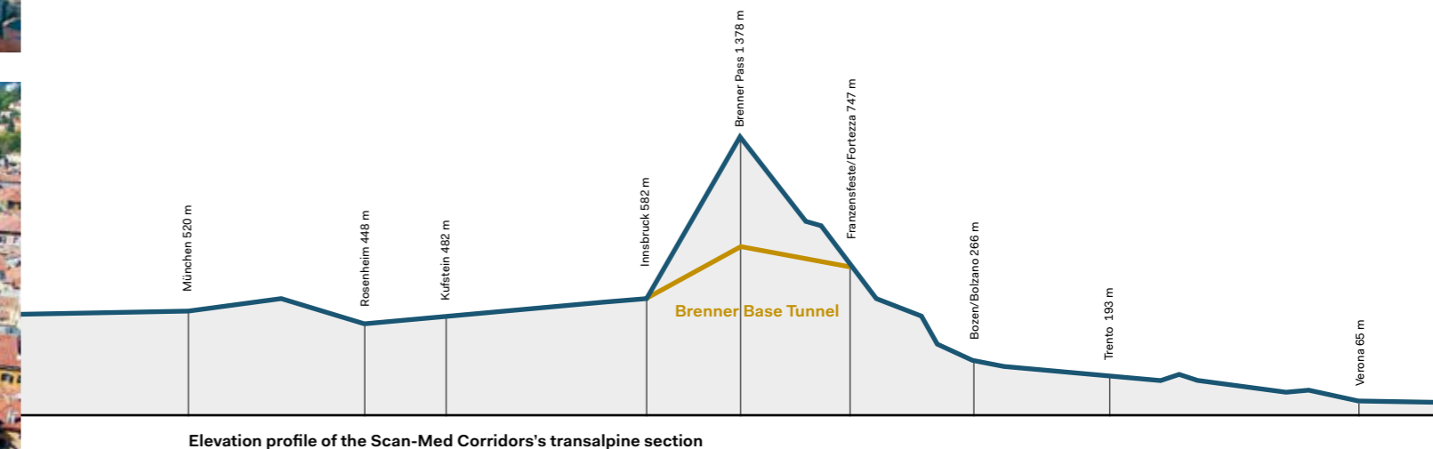
Elevation profile of the Scan-Med Corridor's transalpine section
