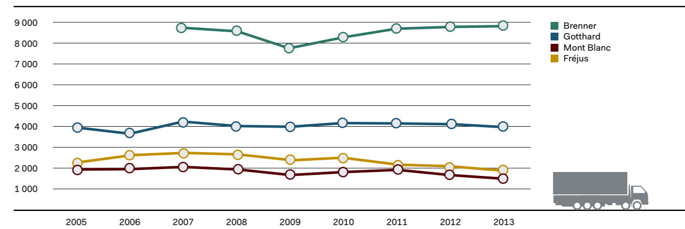
Development of average daily traffic, amount of heavy-duty vehicles (2005-2013)
